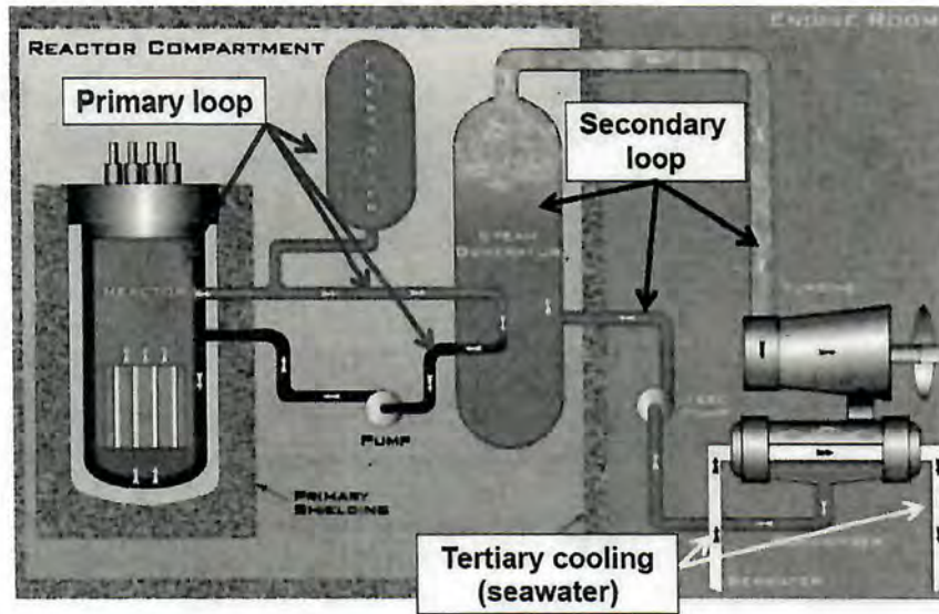
Figure 3: Schematic of naval pressurized water reactor propulsion plant. The “primary” cooling water, which is pumped through the reactor and through a heat exchanger called the “steam generator.” The steam generator transfers primary-coolant heat to the “secondary” water, which boils. The resulting steam drives a turbine, which in turn drives a load that could include an electrical generator, a propeller shaft, etc. The secondary water gives up its waste heat to seawater through a heat exchanger in the condenser. As long as heat exchangers do not leak, the primary coolant is isolated from the secondary, which is isolated from the seawater. (Adapted from John Barry presentation, June 2016.)
