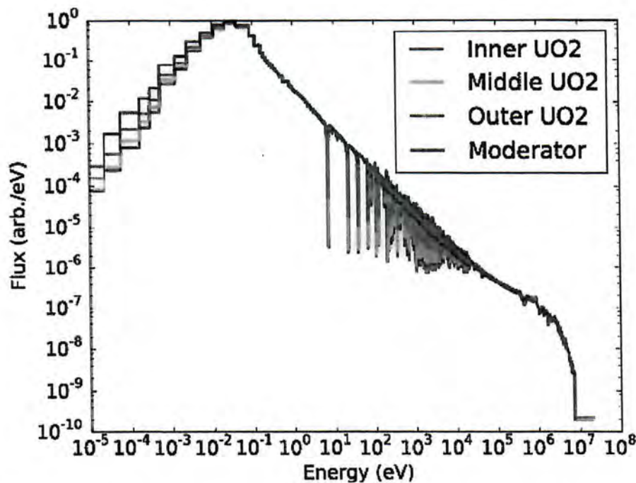
Figure 11: Neutron energy spectrum computed at different positions inside the \text{UO}_2 fuel and the moderator. This shows the position sensitivity of the neutron flux at resonance energies.
